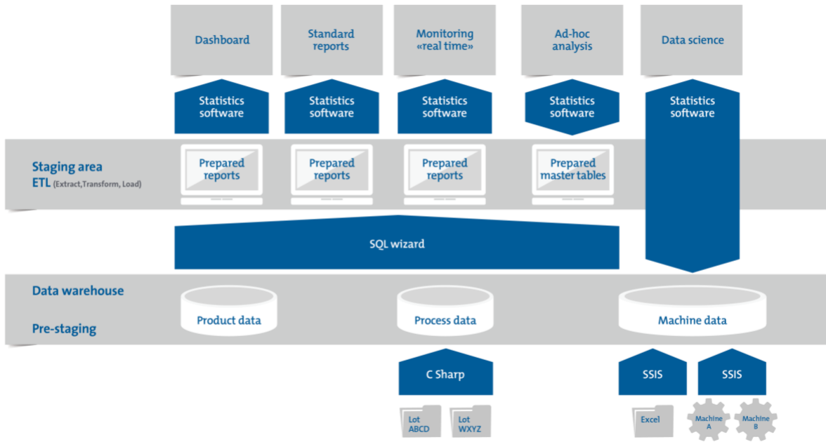
Figure 2. Two-stage DYCO IC2 approach to data processing
